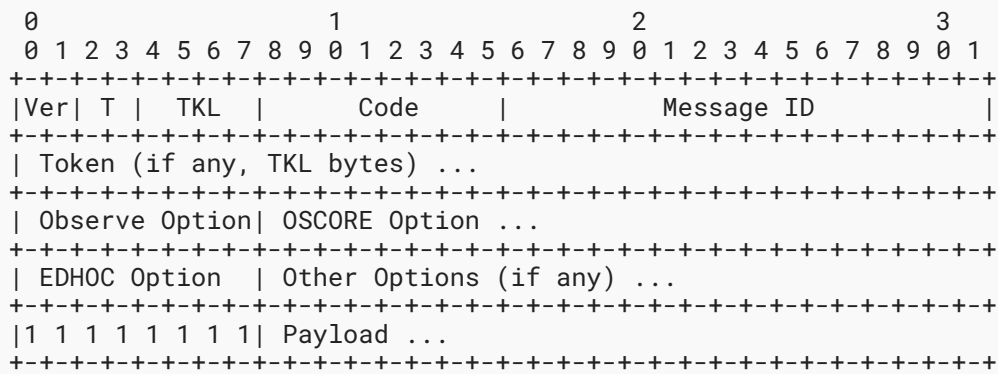
Figure 3: Example of a CoAP Message Containing the Combined EDHOC and OSCORE Data, Signalled by the EDHOC Option and Transported over UDP
